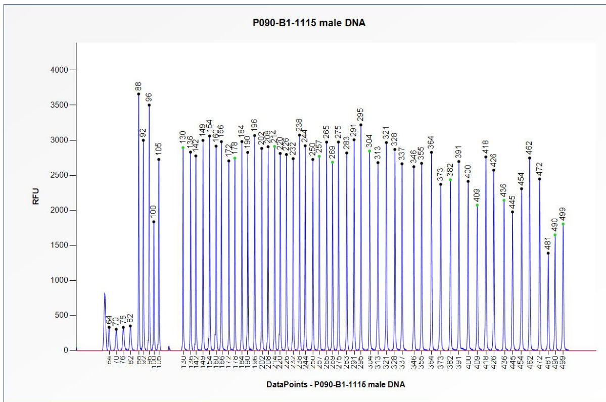
Figure 1. Capillary electrophoresis pattern from a sample of approximately 50 ng human male control DNA analysed with SALSA MLPA Probemix P090 BRCA2 (B1-1115).
