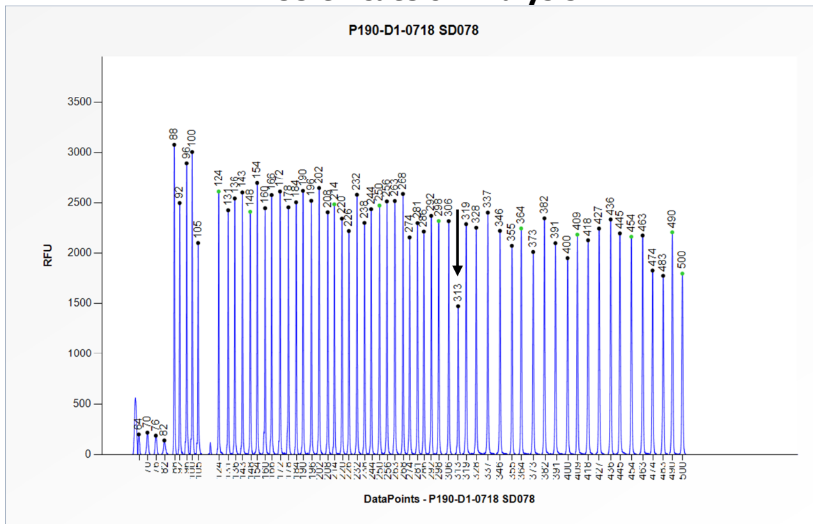
Figure 2. Capillary electrophoresis pattern of SALSA Binning DNA SD078 (approximately 50 ng) analysed with SALSA MLPA probemix P190 CHEK2 (D1-0718). The location of the CHEK2 1100delC mutation specific probe at 313 nt is indicated.
