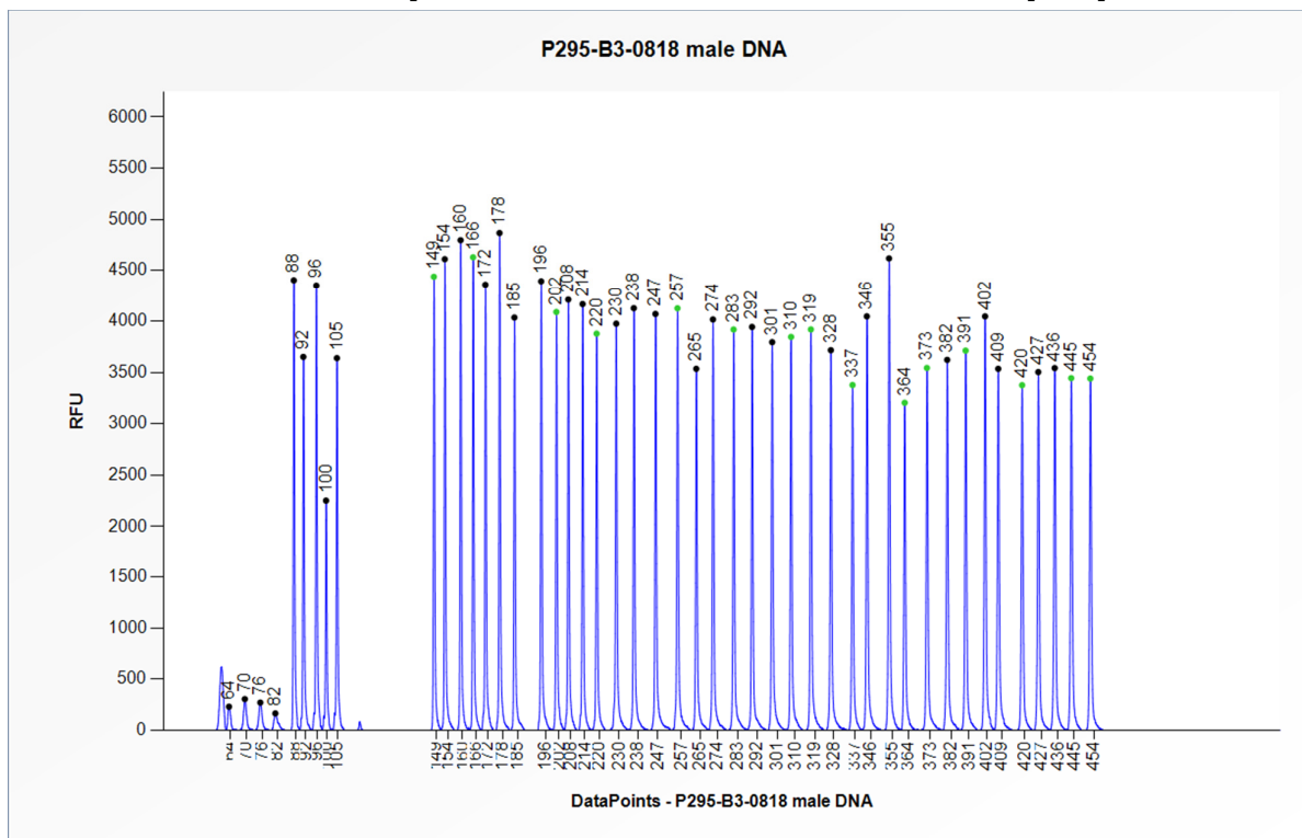
Figure 1. Capillary electrophoresis pattern from a sample of approximately 50 ng human male control DNA analysed with SALSA MLPA probemix P295 SPRED1 (B3-0818).
