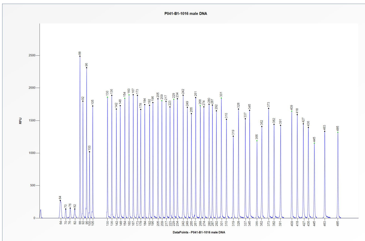
Figure 1. Capillary electrophoresis pattern from a sample of approximately 50 ng human male control DNA analysed with SALSA MLPA probemix P041 ATM-1 (B1-1016).
