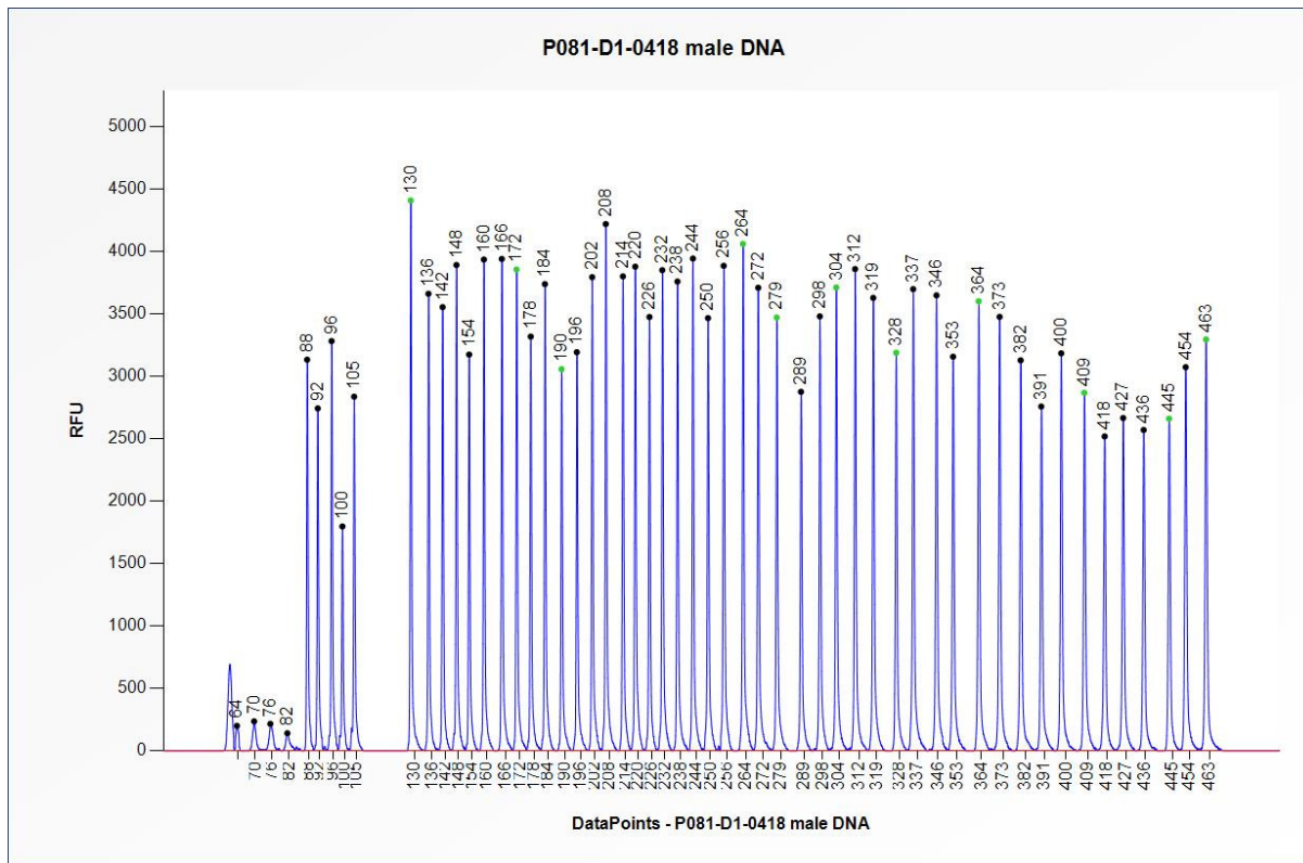
Figure 1. Capillary electrophoresis pattern from a sample of approximately 50 ng human male control DNA analysed with SALSA MLPA probemix P081 NF1 mix 1 (D1-0418).
