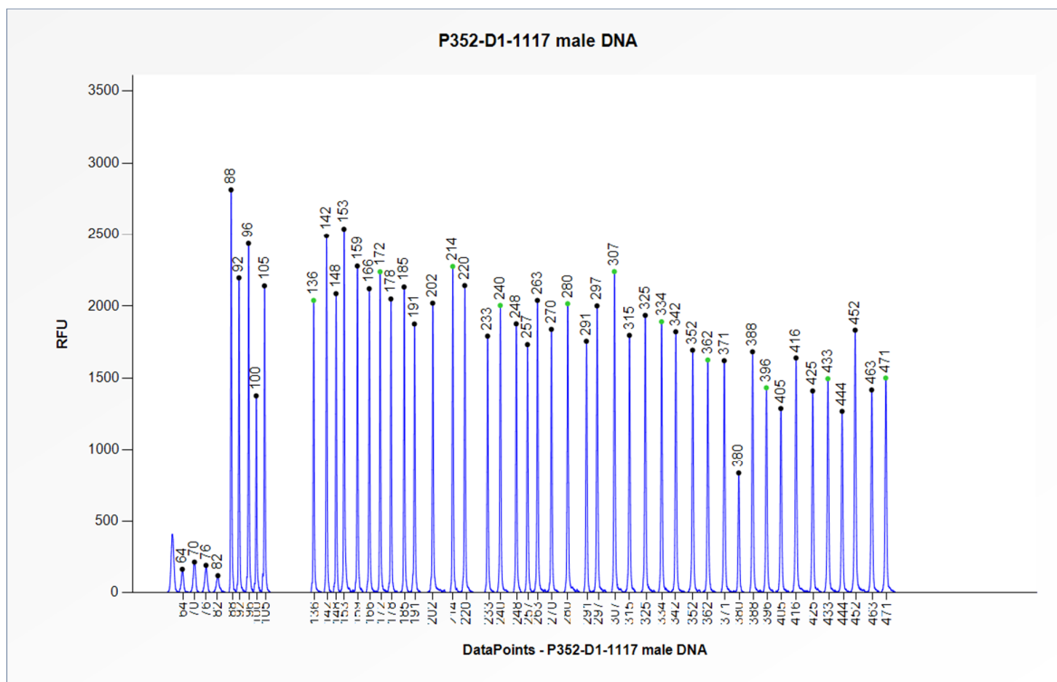
Figure 1. Capillary electrophoresis pattern from a sample of approximately 50 ng human male control DNA analysed with SALSA MLPA probemix P352 PKD1-PKD2 (D1-1117).
