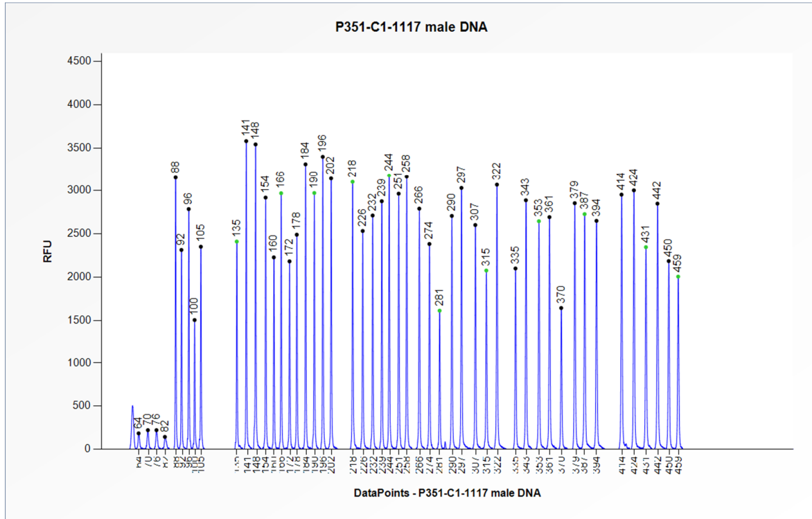
Figure 1. Capillary electrophoresis pattern from a sample of approximately 50 ng human male control DNA analysed with SALSA MLPA probemix P351 PKD1 (C1-1117).
